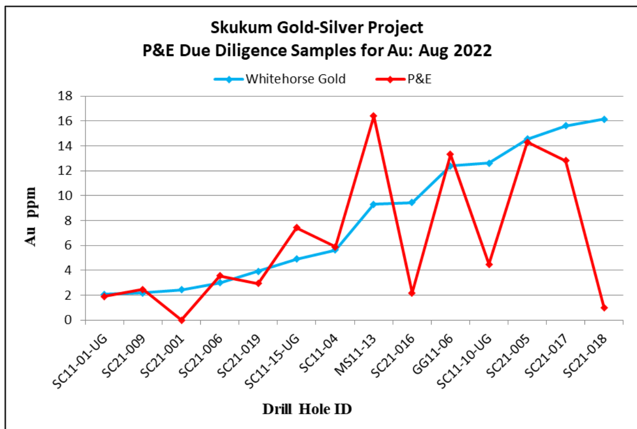
FIGURE 12.1 P&E SITE VISIT RESULTS: AU
