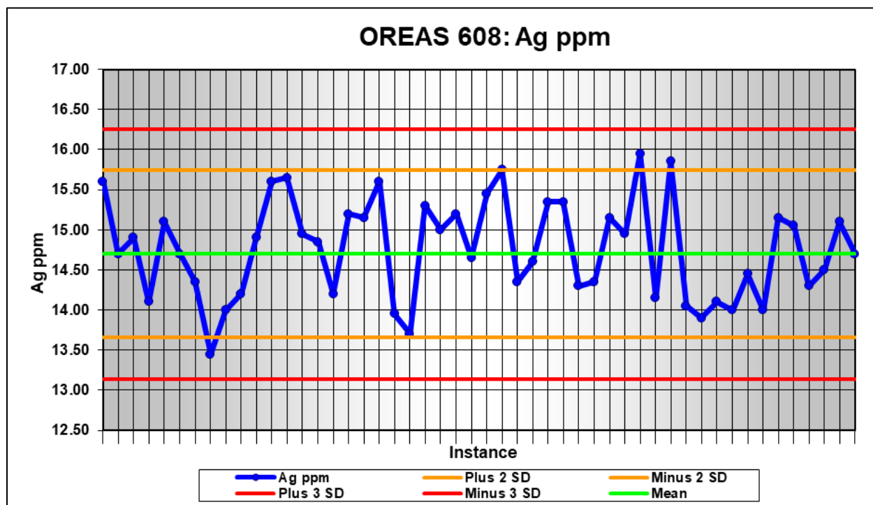
FIGURE 11.8 PERFORMANCE OF OREAS 608 CRM: AG
