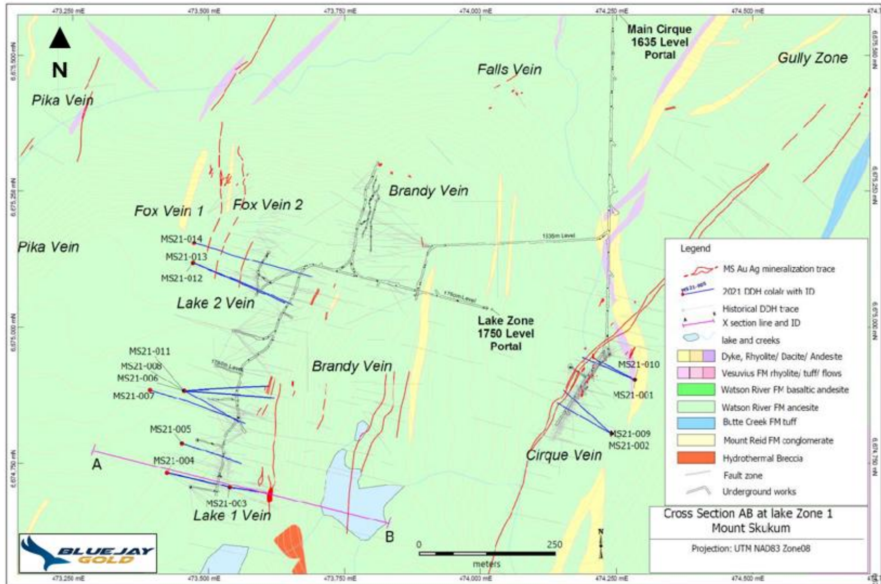
FIGURE 10.8 PLAN VIEW OF THE MT. SKUKUM DEPOSIT AREA
