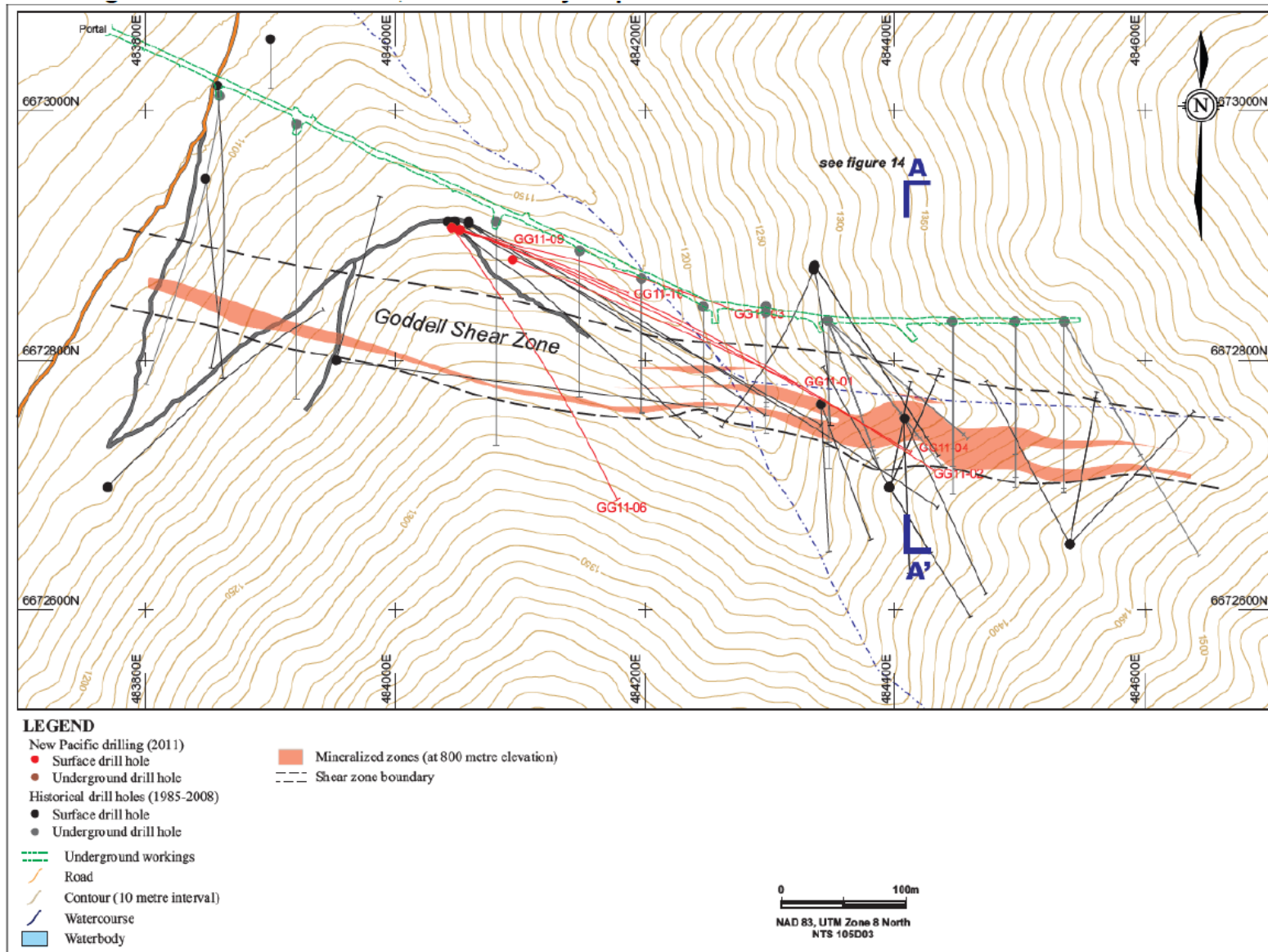
FIGURE 6.6 GODDELL GULLY 2011 DRILL HOLE PLAN
