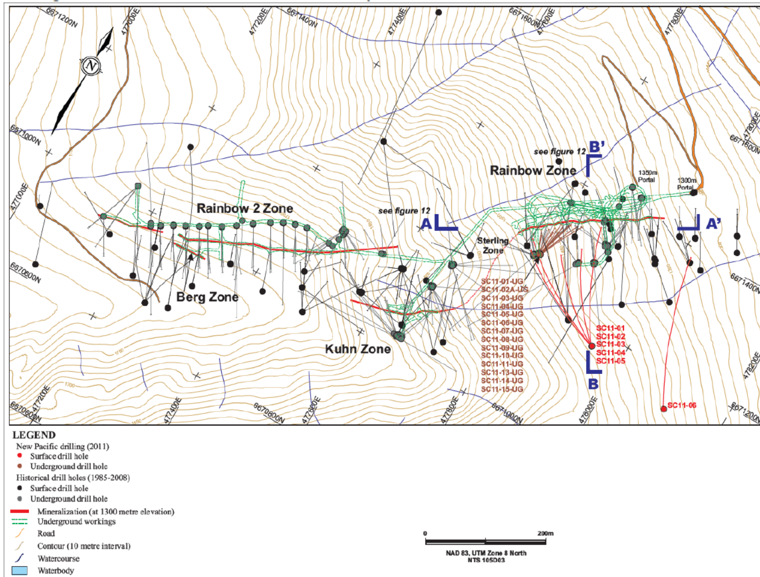
FIGURE 6.4 SKUKUM CREEK DEPOSIT 2011 DRILL HOLE PLAN
