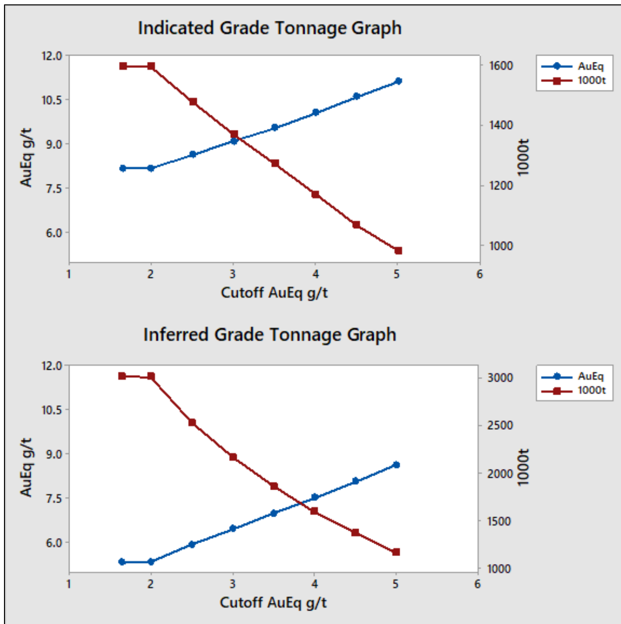
FIGURE 14.8 GRADE SENSITIVITY FOR INDICATED AND INFERRED MINERAL RESOURCES
