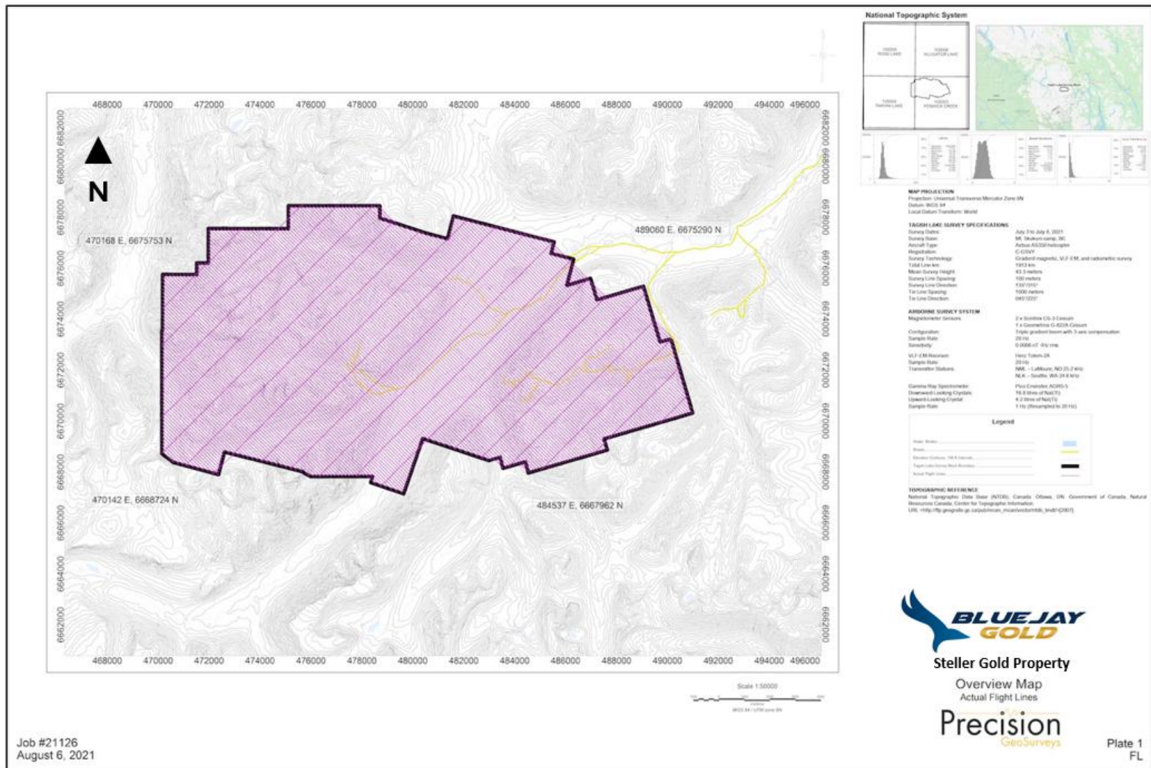
FIGURE 9.4 FLIGHT LINES FOR 2021 AIRBORNE GEOPHYSICAL SURVEY
