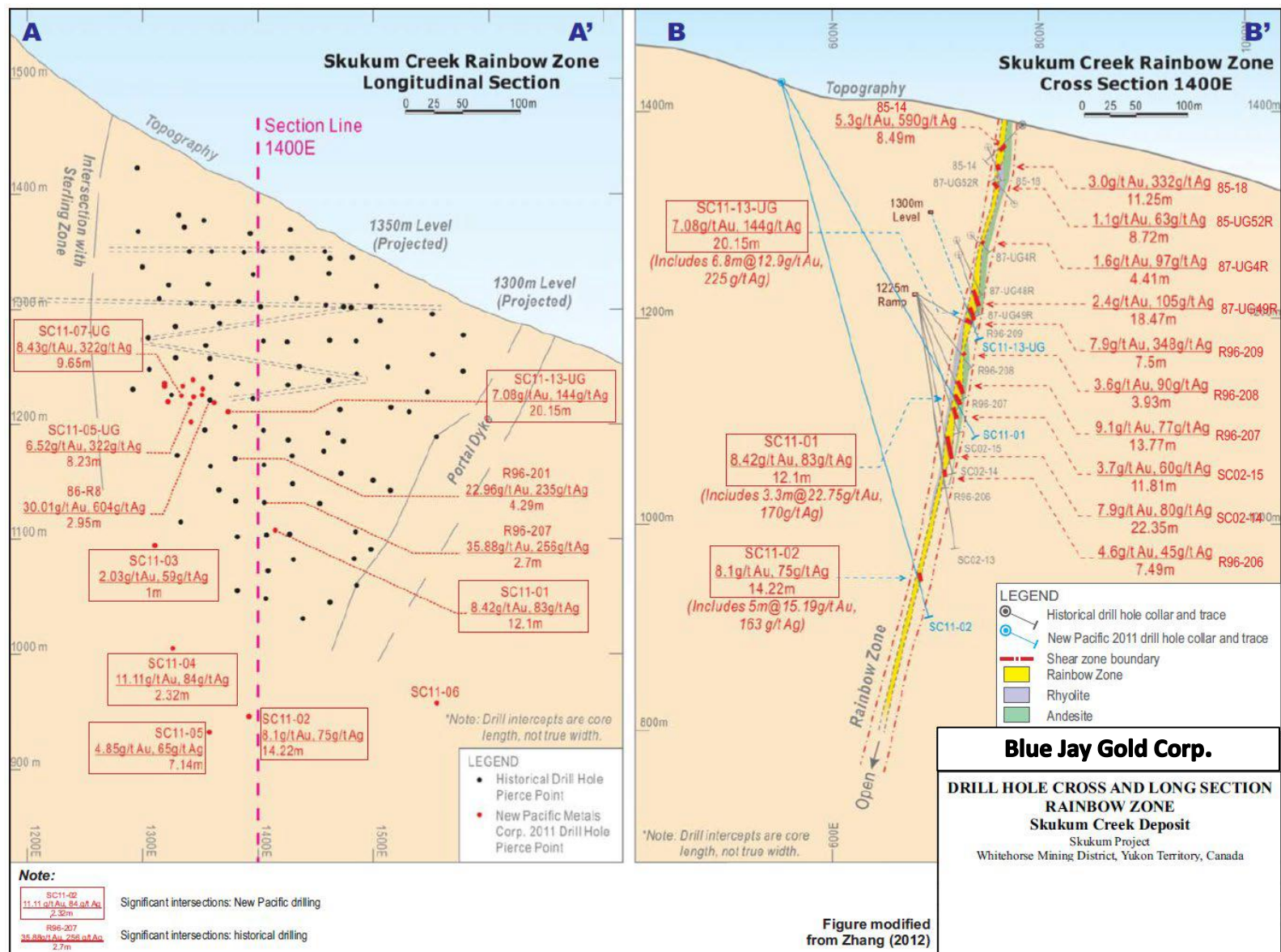
FIGURE 6.5 SKUKUM CREEK 2011 DRILL HOLE LONGITUDINAL AND CROSS-SECTIONAL PROJECTIONS
