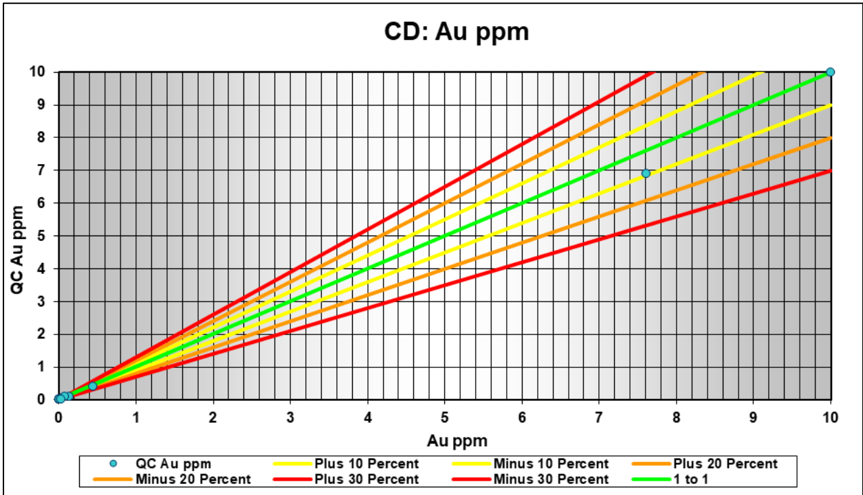
FIGURE 11.15 COARSE REJECT DUPLICATE SCATTER PLOT: AU
