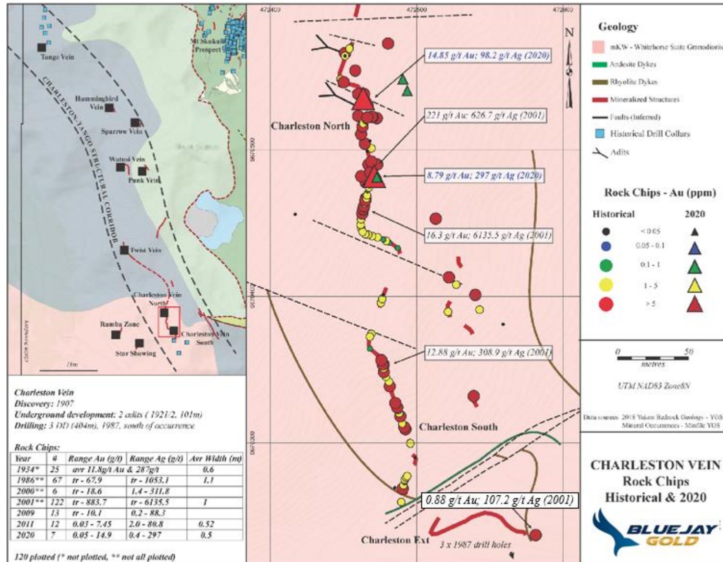
FIGURE 9.1 CHARLESTON VEIN SAMPLING, 2020 AND HISTORICAL SAMPLING
