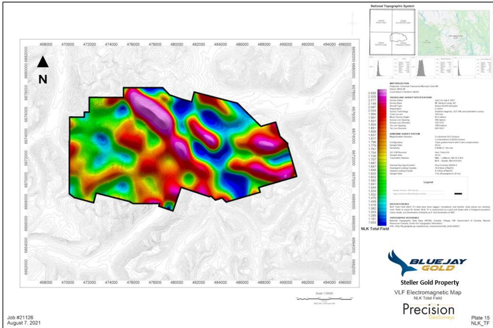
FIGURE 9.8 VLF ELECTROMAGNETIC MAP
