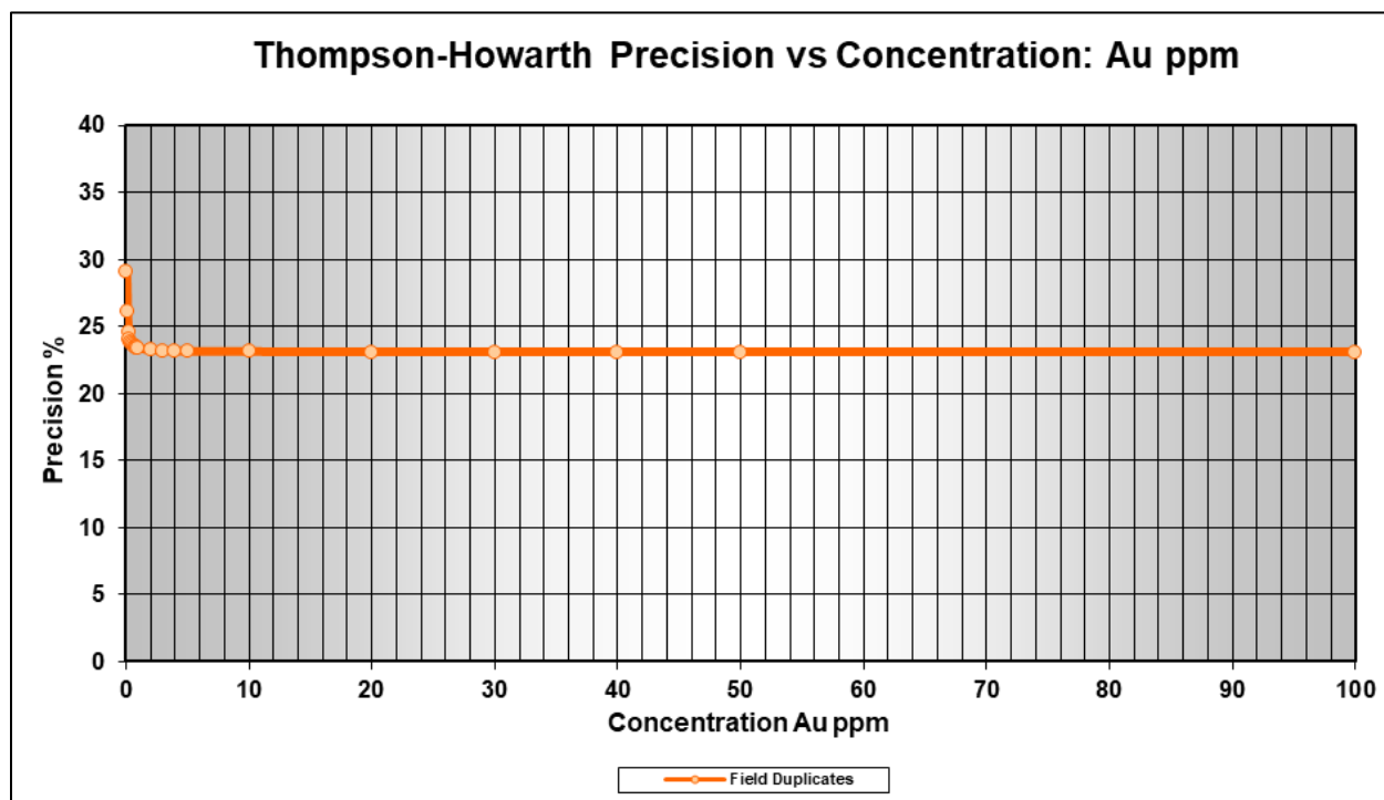
FIGURE 11.12 FIELD DUPLICATE THOMPSON-HOWARTH PLOT: AU
