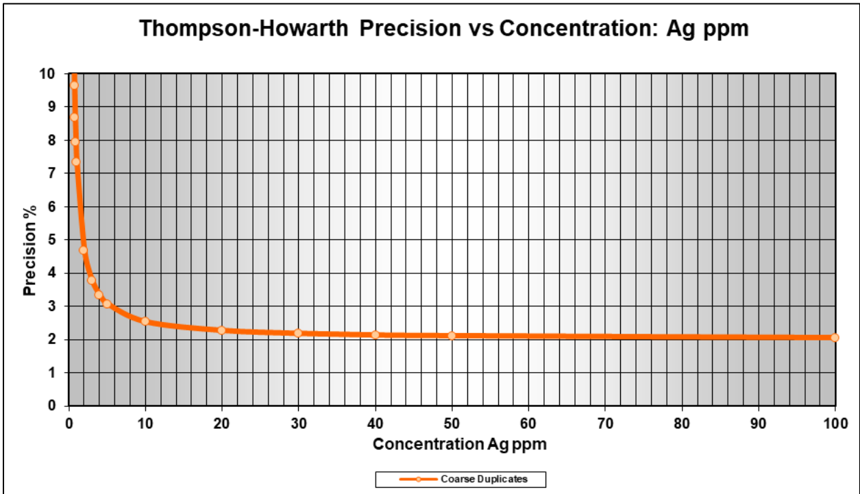
FIGURE 11.18 COARSE REJECT DUPLICATE THOMPSON-HOWARTH PLOT: AG
