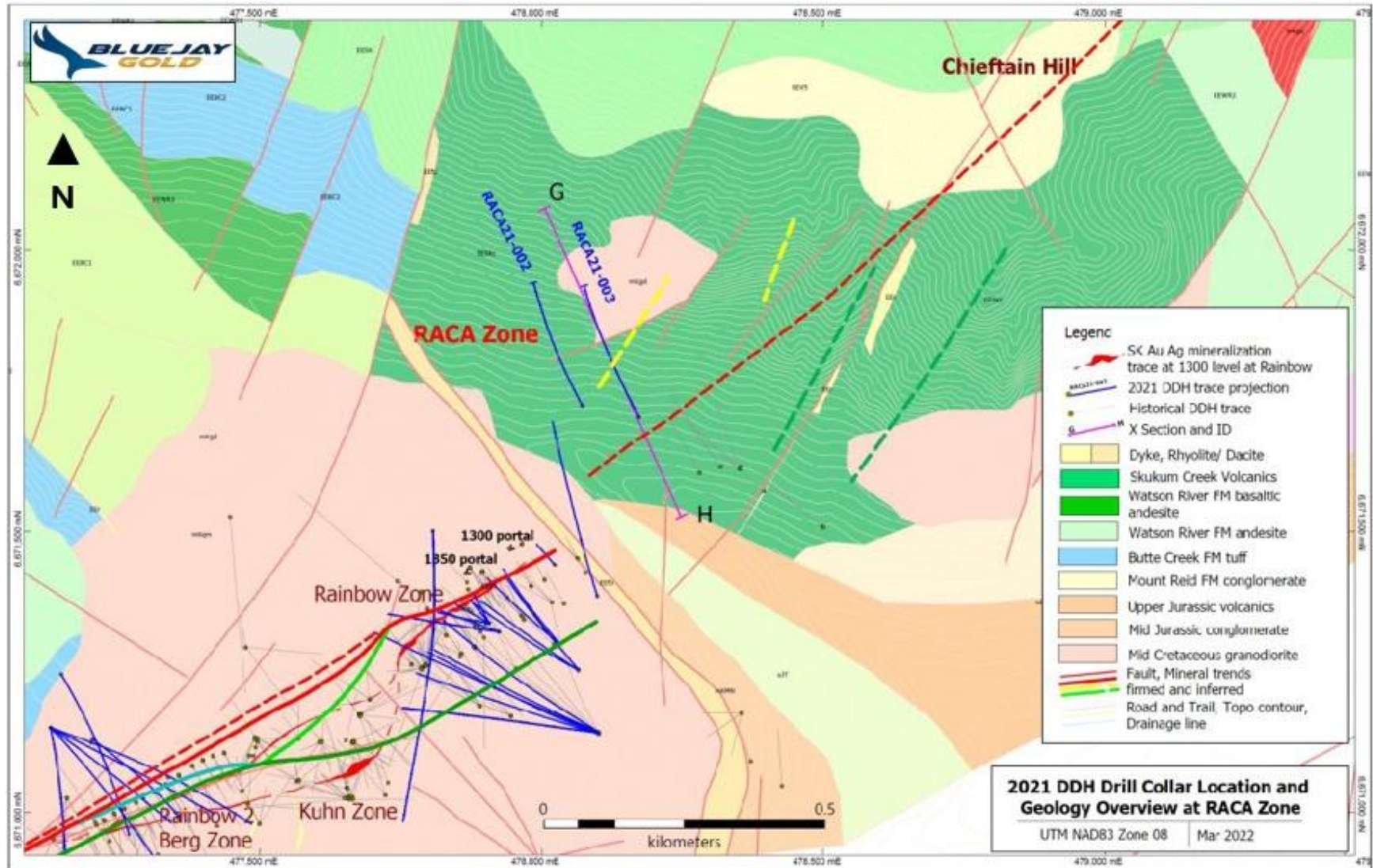
FIGURE 10.6 PLAN VIEW OF THE RACA ZONE
