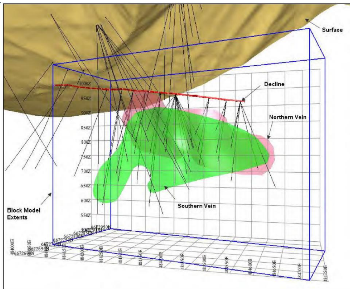
FIGURE 7.7 GODDELL GULLY DEPOSIT 3-D ISOMETRIC VIEW
