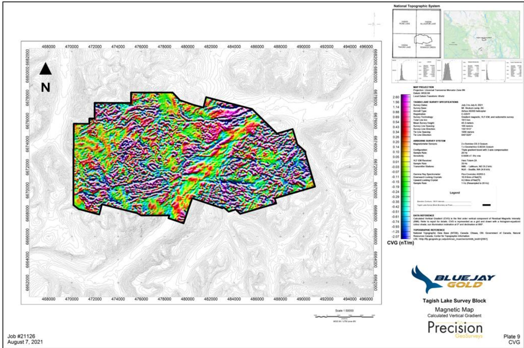
FIGURE 9.7 CALCULATED VERTICAL GRADIENT AIRBORNE MAGNETIC MAP
