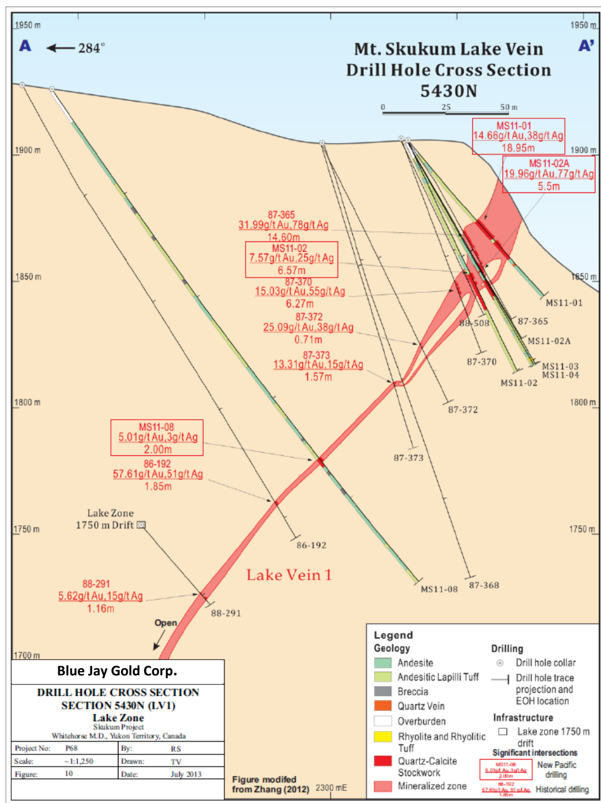
FIGURE 6.3 2011 LAKE ZONE (LV1) DRILL HOLE CROSS-SECTIONAL PROJECTION 5340N
