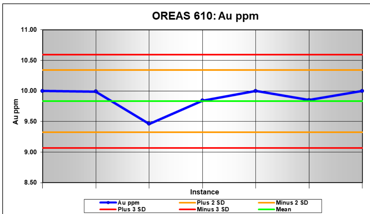
FIGURE 11.9 PERFORMANCE OF OREAS 610 CRM: AU
