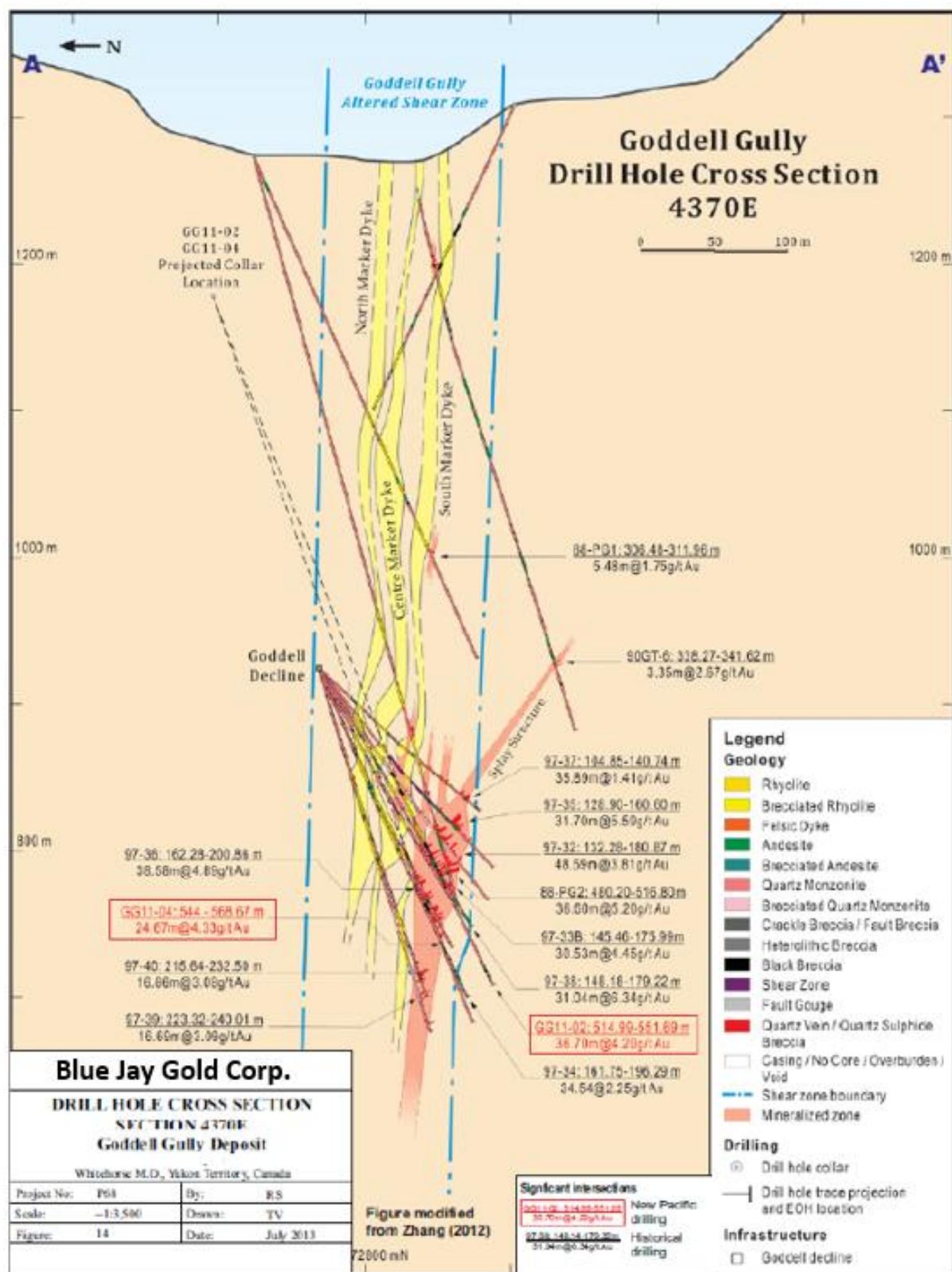
FIGURE 6.7 GODDELL GULLY 2011 DRILL HOLE CROSS-SECTIONAL PROJECTION 4370E
