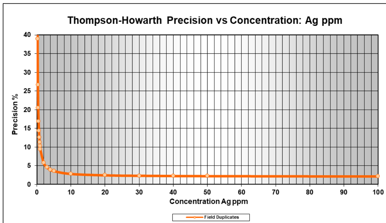
FIGURE 11.14 FIELD DUPLICATE THOMPSON-HOWARTH PLOT: AG
