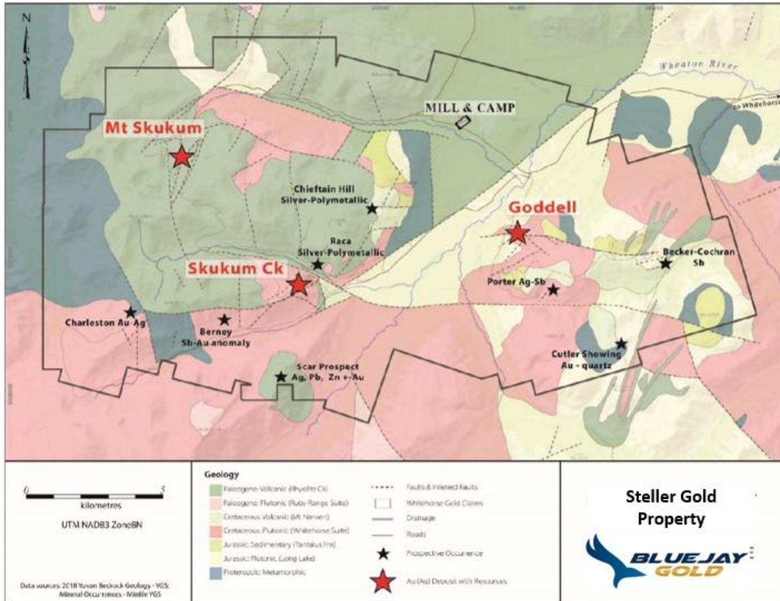
FIGURE 10.2 PROJECT OVERVIEW MAP HIGHLIGHTING THE THREE MAIN MINERAL RESOURCE AREAS
