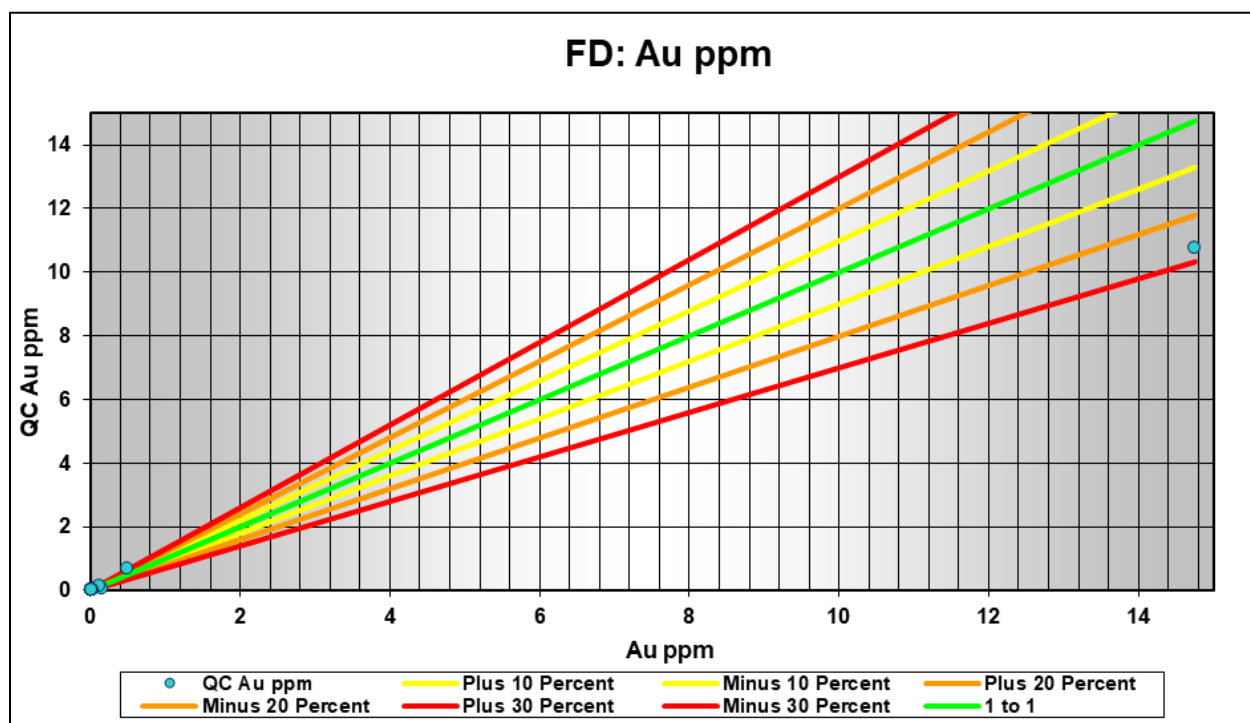
FIGURE 11.11 FIELD DUPLICATE SCATTER PLOT: AU
