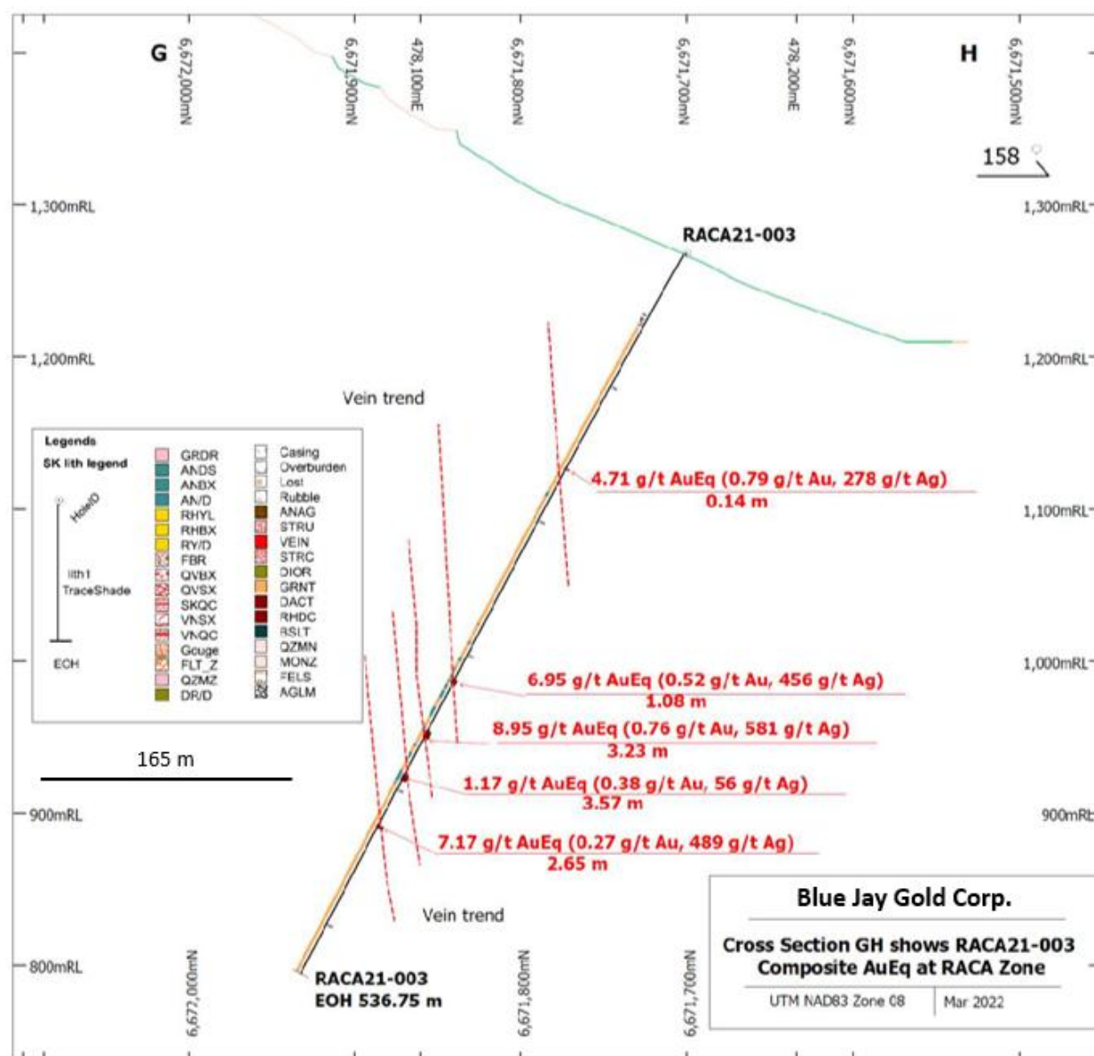
FIGURE 10.7 RACA ZONE VERTICAL CROSS-SECTION G-H
