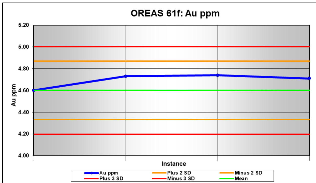
FIGURE 11.1 PERFORMANCE OF OREAS 61F CRM: AU
