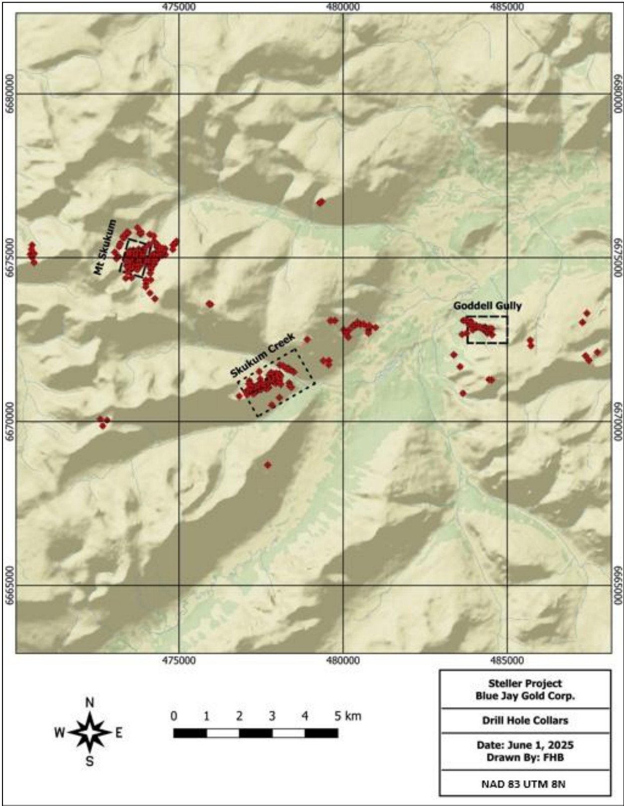
FIGURE 14.1 DRILL HOLE LOCATIONS
