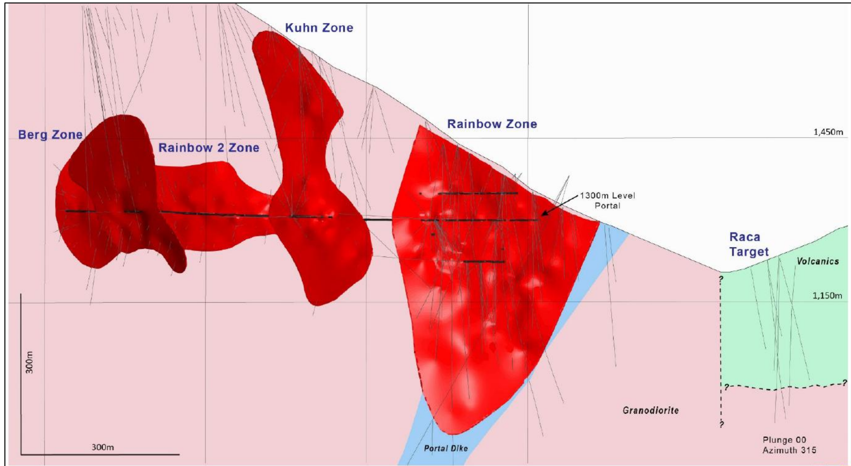
FIGURE 7.5 SKUKUM CREEK LONGITUDINAL PROJECTION
