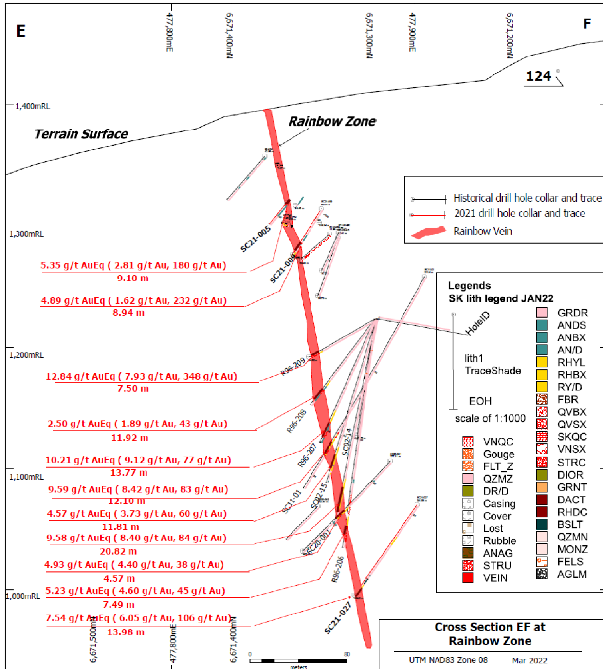
FIGURE 10.4 VERTICAL CROSS-SECTION PROJECTION E-F ON THE RAINBOW ZONE SHOWING 2021 AND HISTORICAL DRILL HOLE INTERCEPTS
