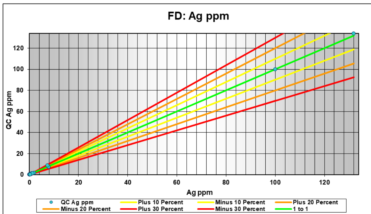
FIGURE 11.13 FIELD DUPLICATE SCATTER PLOT: AG
