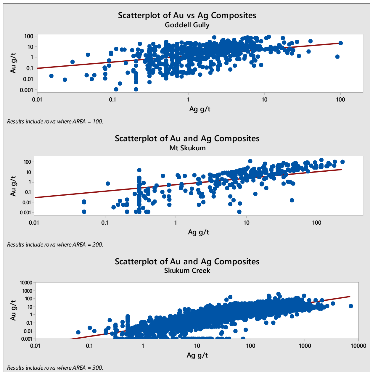
FIGURE 14.3 AU AND AG CORRELATION
