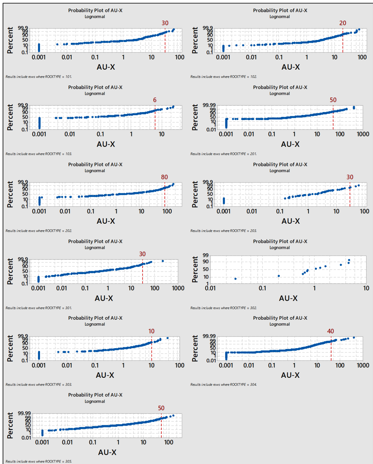
FIGURE 14.5 AU COMPOSITES LOG-PROBABILITY PLOTS
