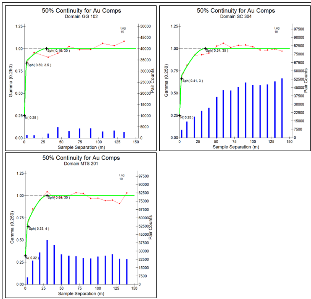
FIGURE 14.7 SEMI-VARIOGRAMS
