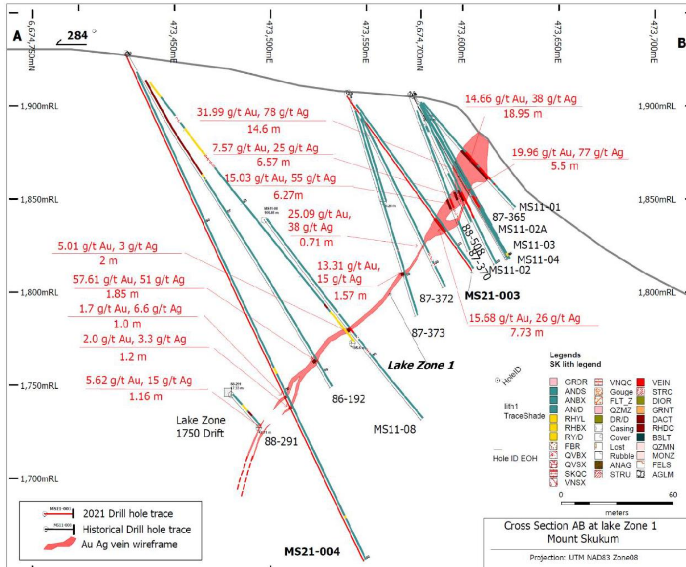
FIGURE 10.9 VERTICAL CROSS-SECTION PROJECTION OF THE MT. SKUKUM ZONE
