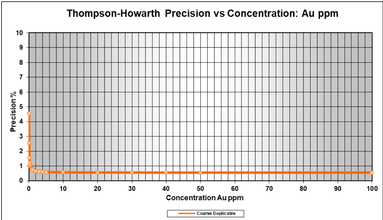
FIGURE 11.16 COARSE REJECT DUPLICATE THOMPSON-HOWARTH PLOT: AU
