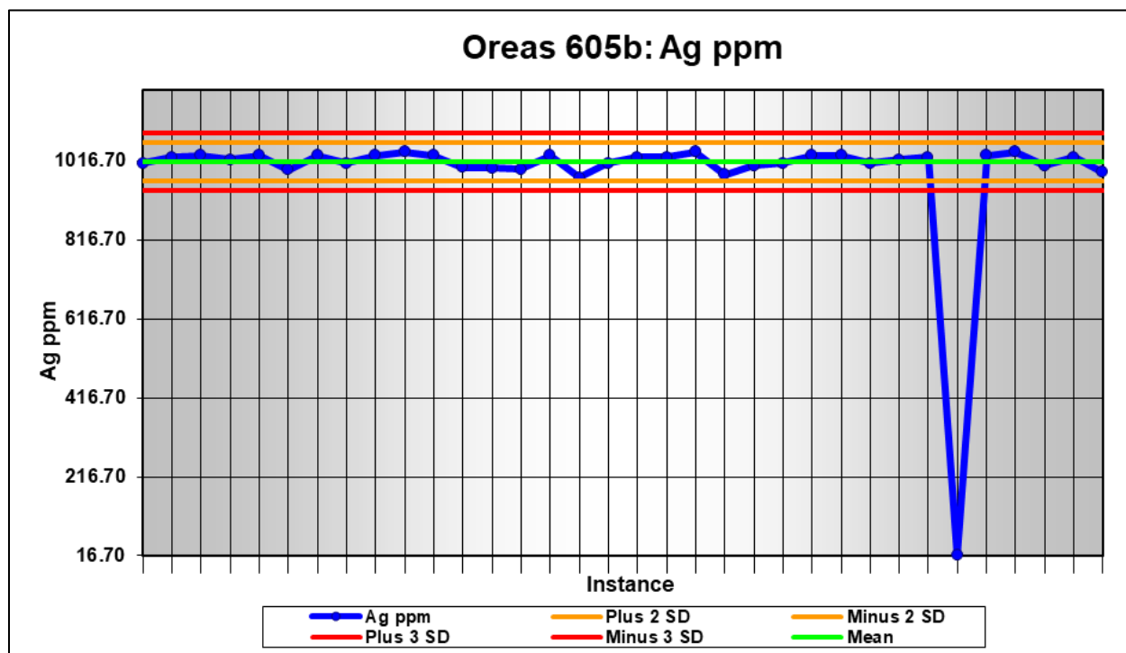
FIGURE 11.6 PERFORMANCE OF OREAS 605B CRM: AG
