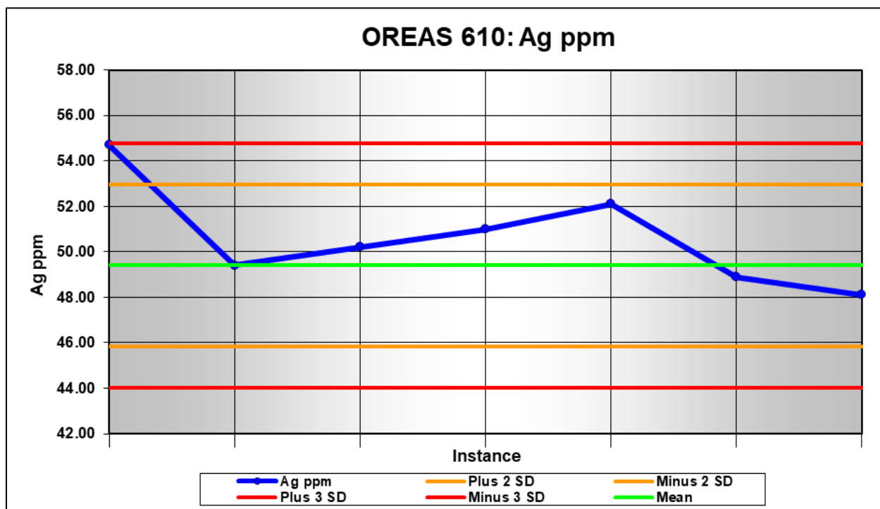
FIGURE 11.10 PERFORMANCE OF OREAS 610 CRM: AG
