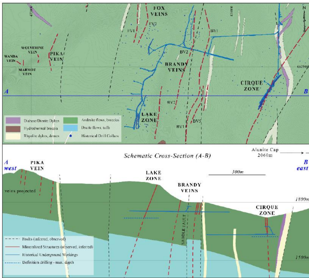
FIGURE 7.4 MT. SKUKUM DEPOSIT CROSS-SECTIONAL PROJECTION
