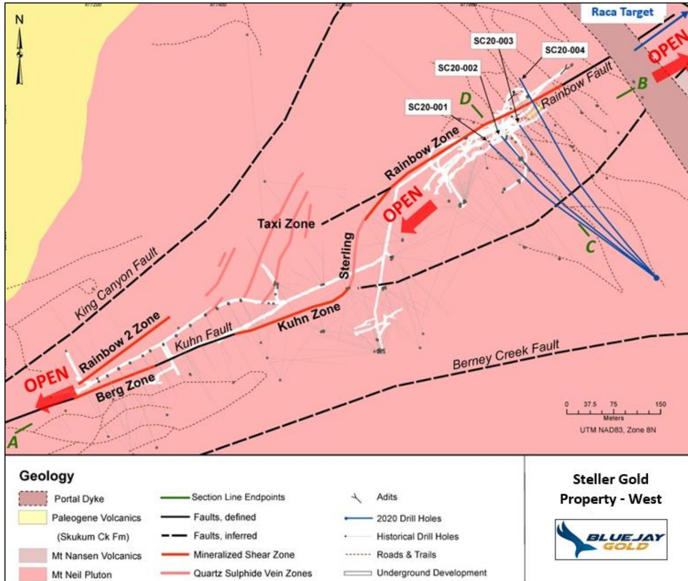
FIGURE 10.1 DIAMOND DRILL HOLE LOCATIONS 2020 DRILL PROGRAM
