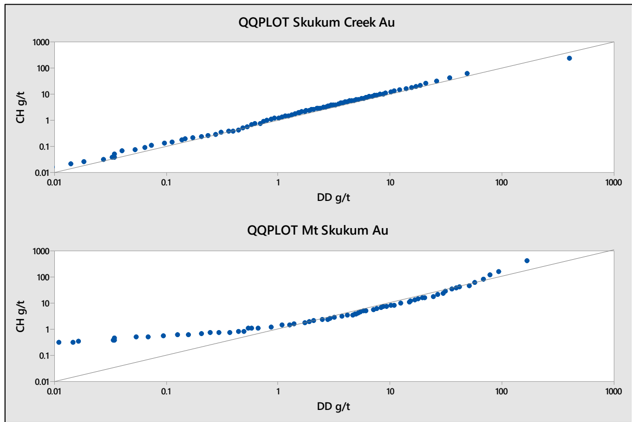
FIGURE 14.4 QQ PLOTS
