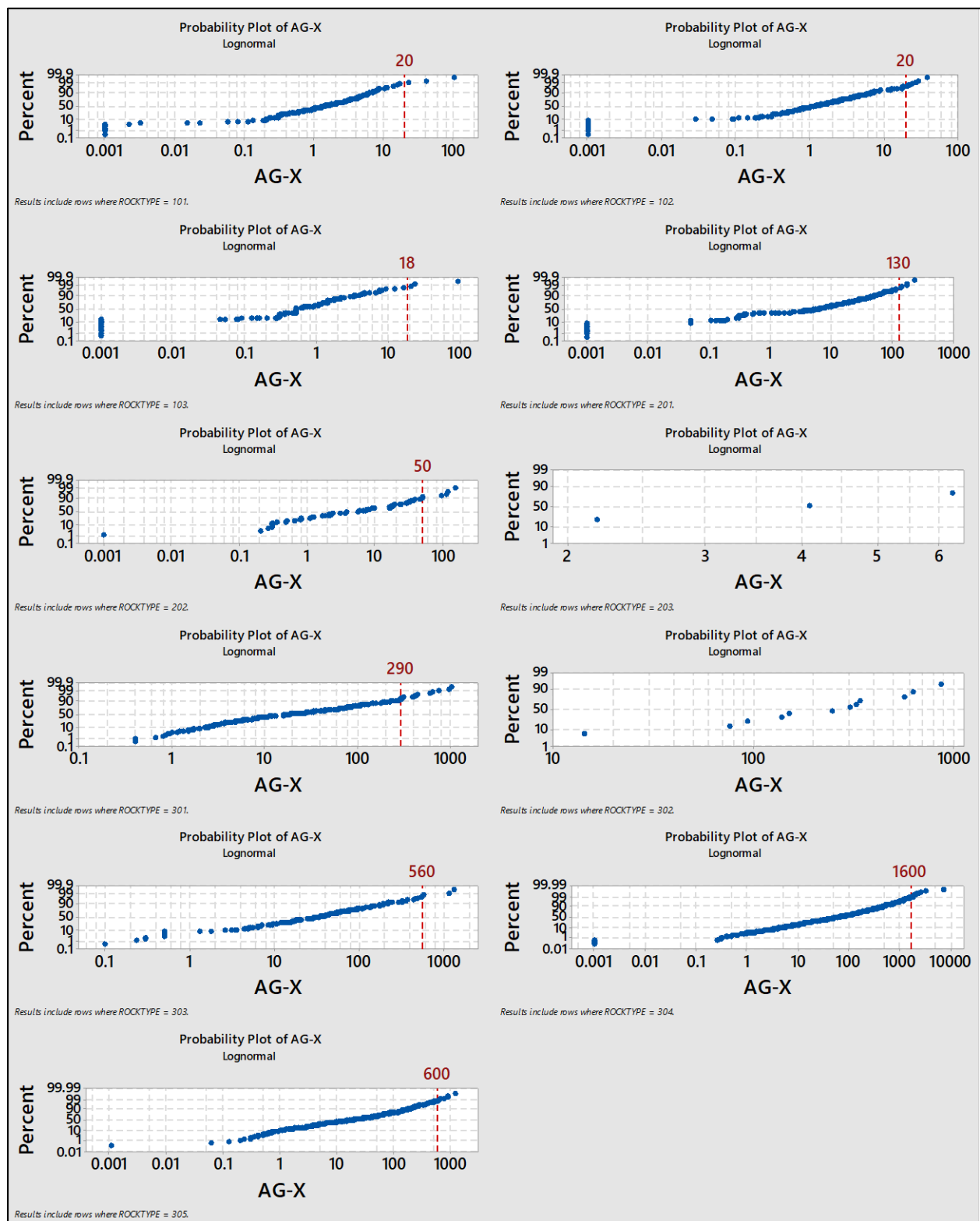
FIGURE 14.6 AG COMPOSITES LOG-PROBABILITY PLOTS
