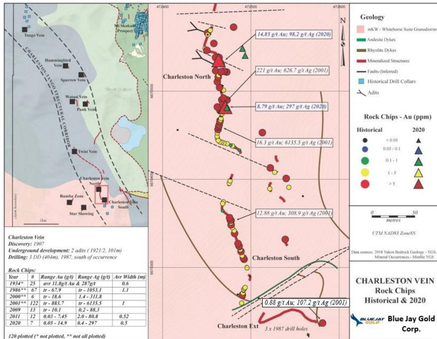
FIGURE 7.8 CHARLESTON DEPOSIT/ZONE GEOLOGY
