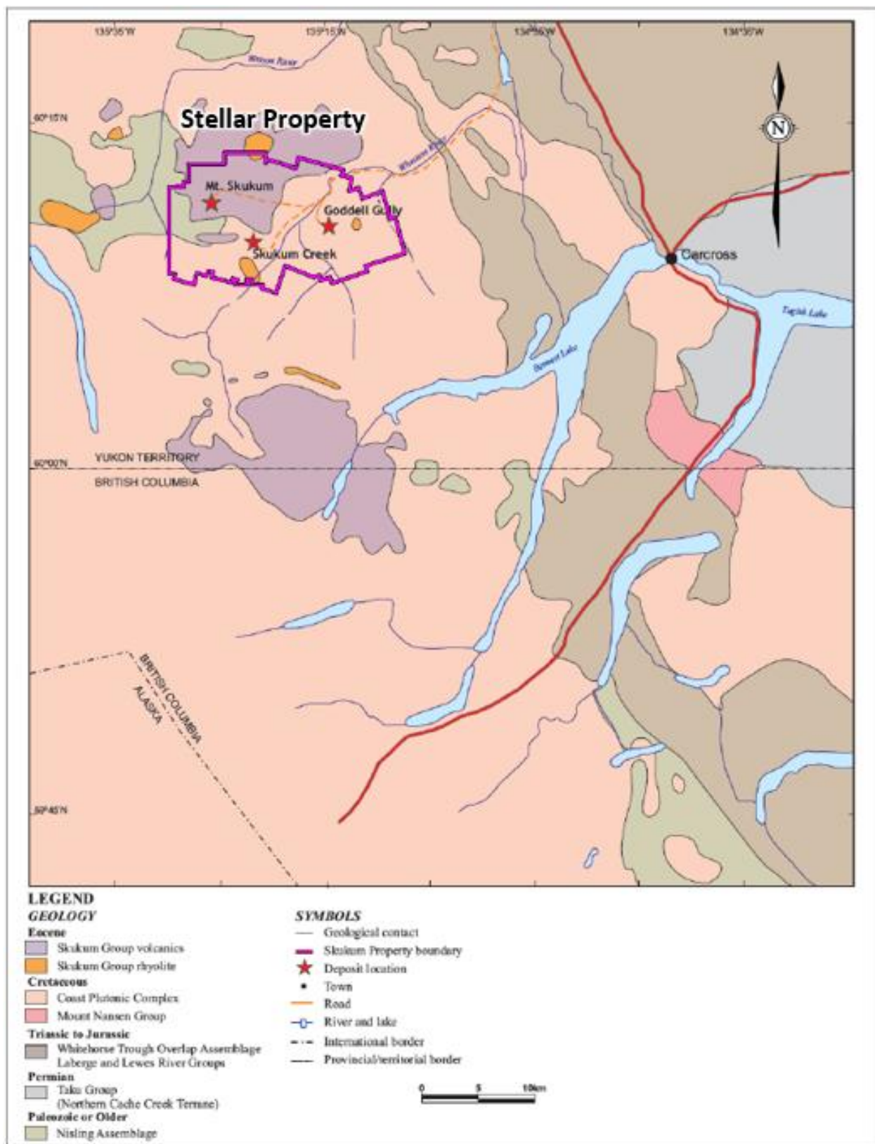
FIGURE 7.1 STELLER PROPERTY REGIONAL GEOLOGICAL SETTING
