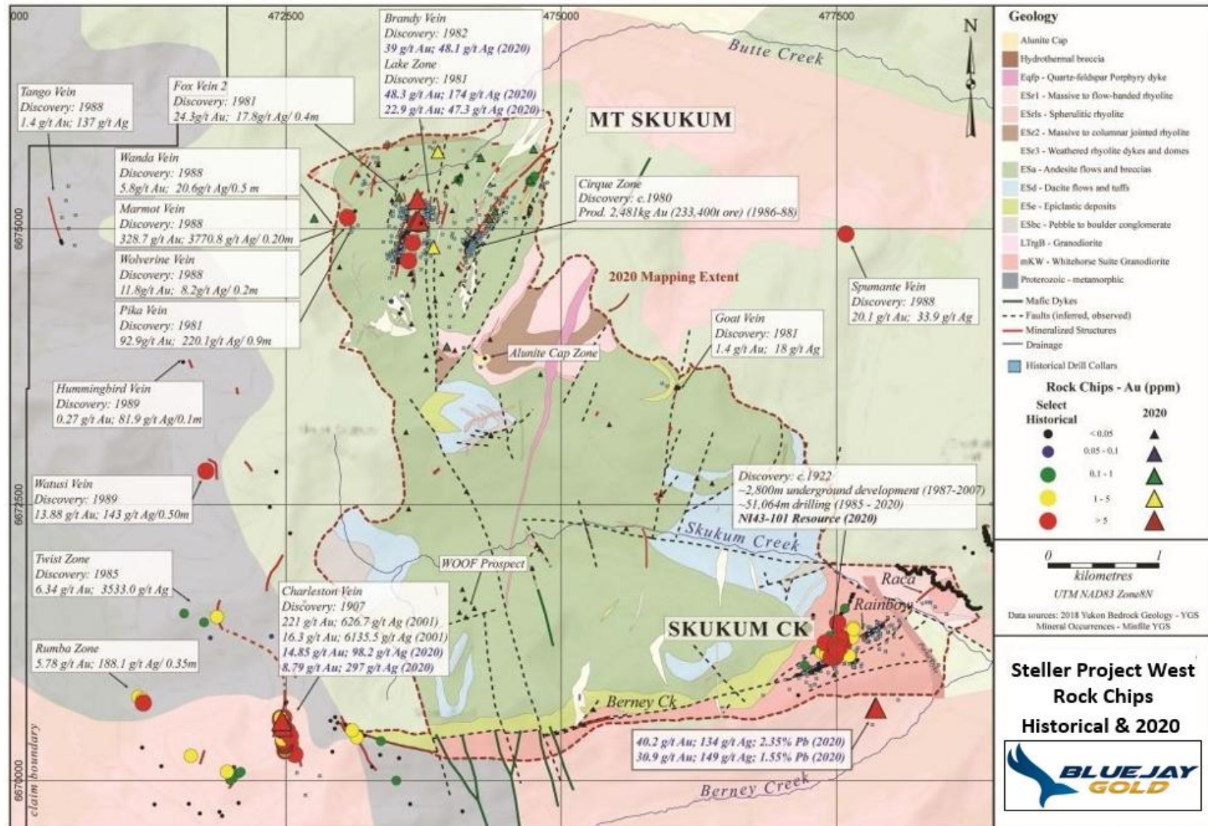
FIGURE 7.3 MT. SKUKUM AND SKUKUM CREEK DEPOSITS AREA GEOLOGY
