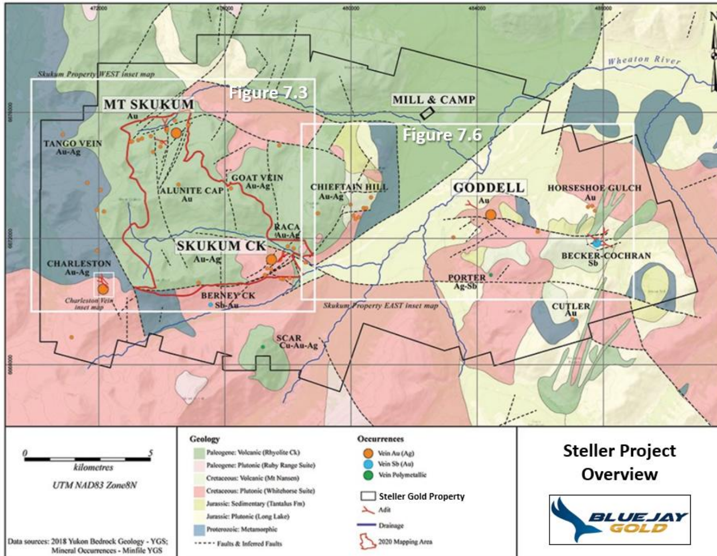
FIGURE 7.2 STELLER PROPERTY GEOLOGY
