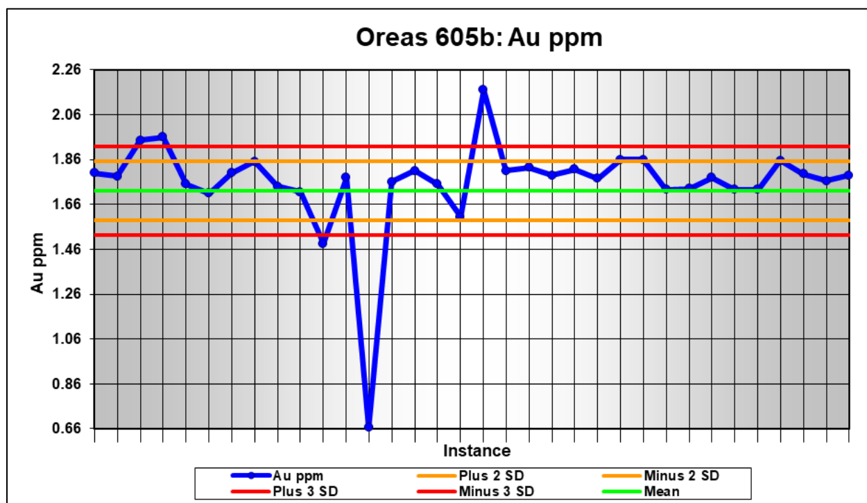
FIGURE 11.5 PERFORMANCE OF OREAS 605B CRM: AU
