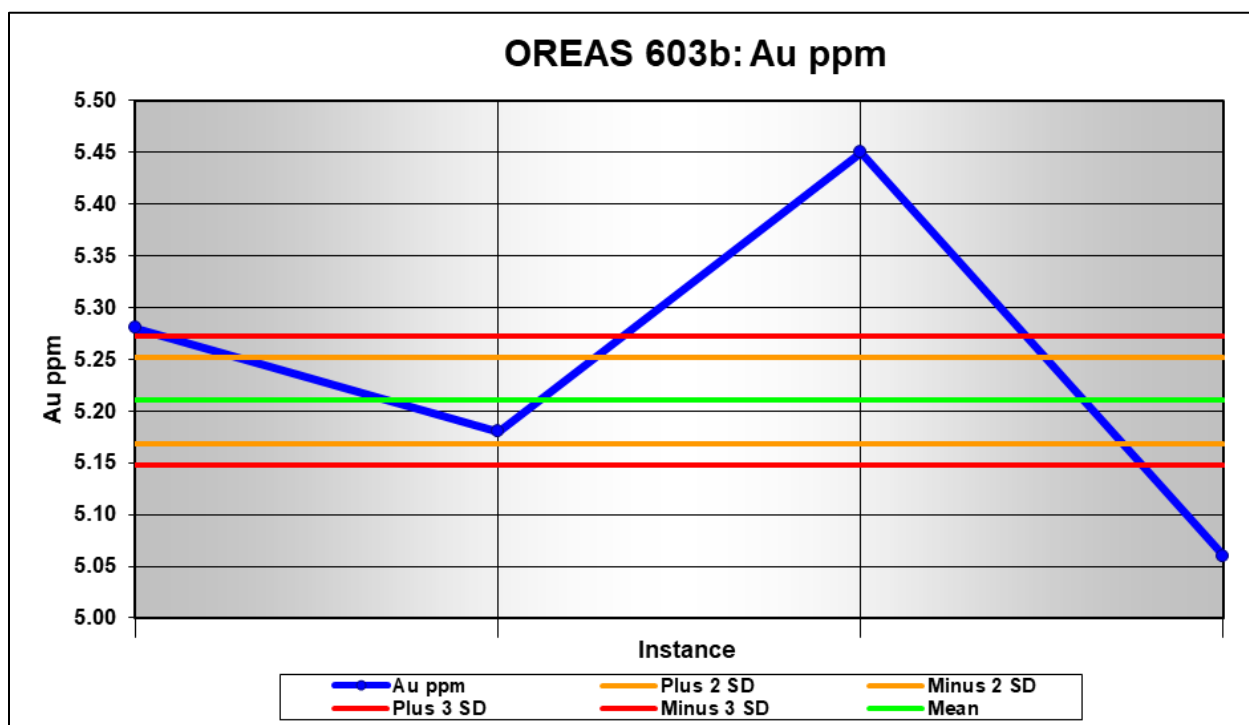
FIGURE 11.3 PERFORMANCE OF OREAS 603B CRM: AU
