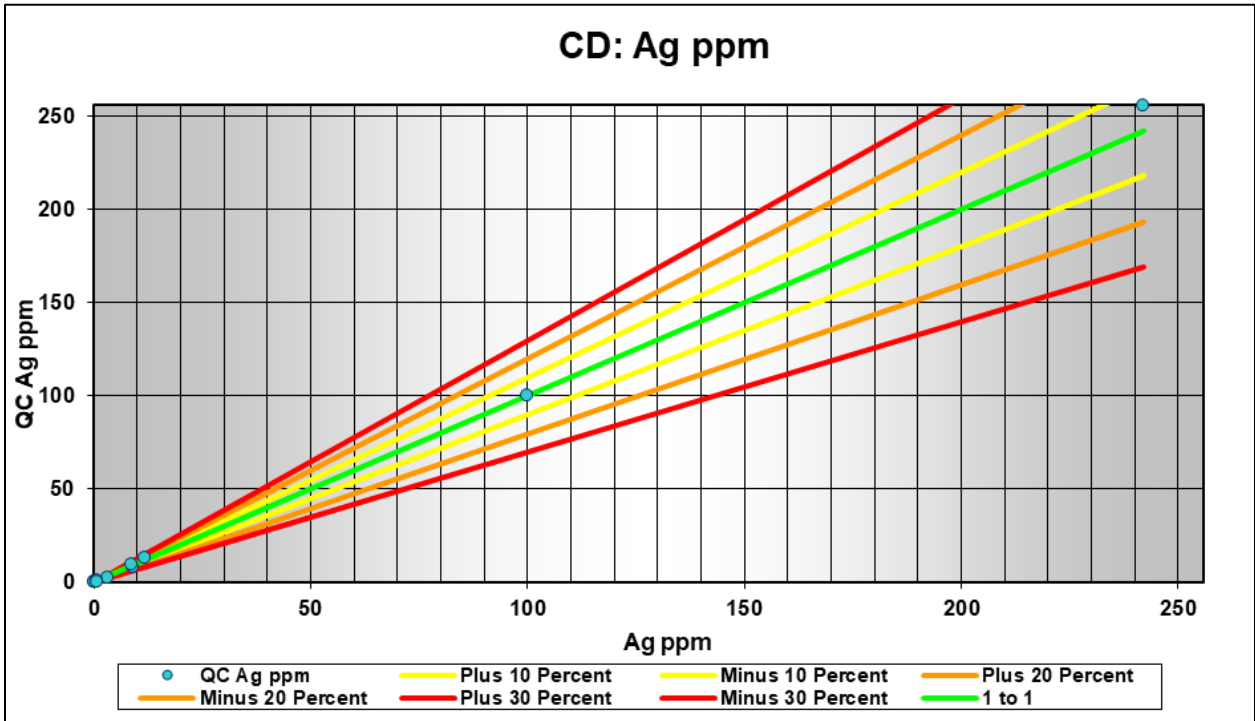
FIGURE 11.11 COARSE REJECT DUPLICATE SCATTER PLOT: AG
