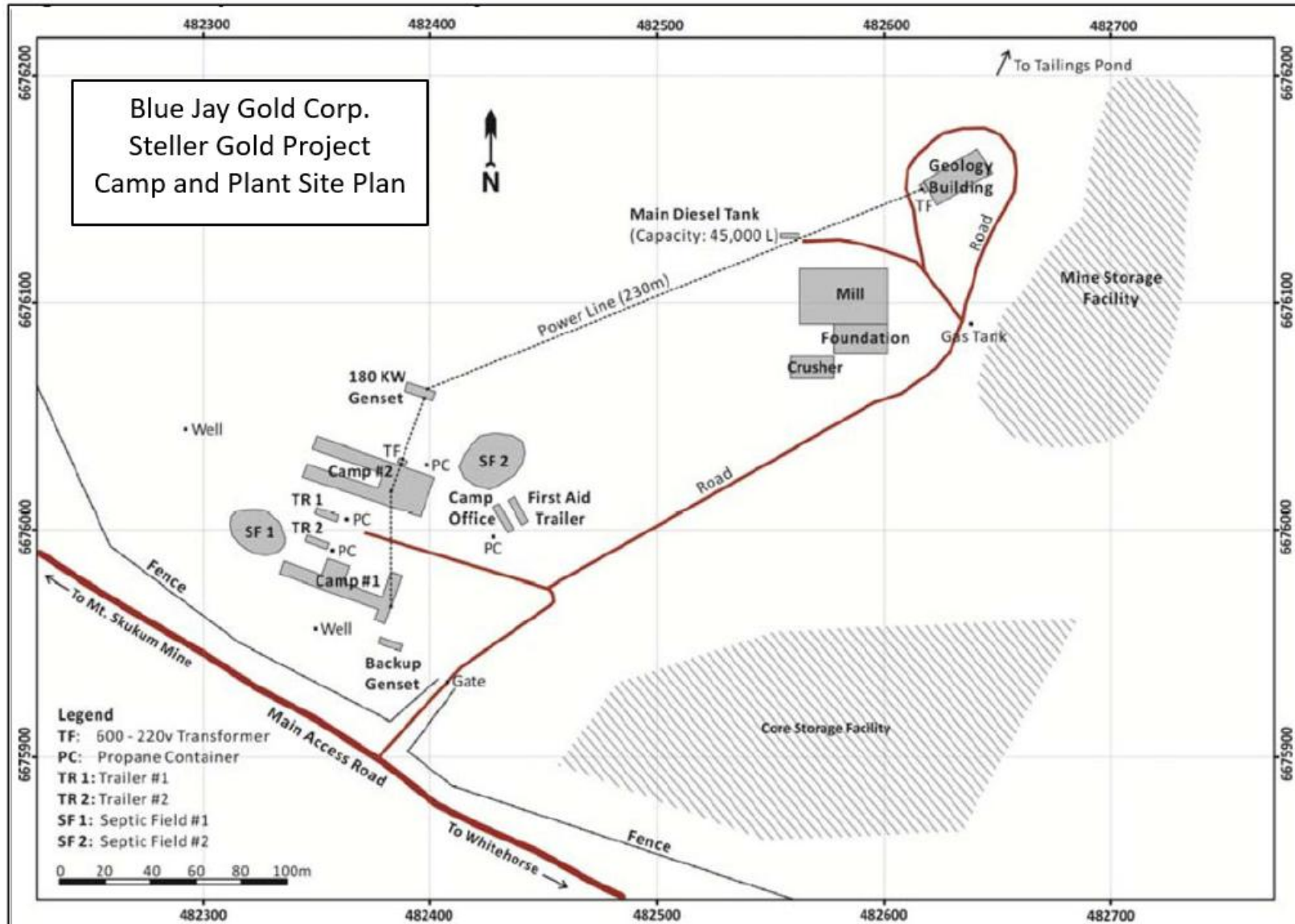
FIGURE 5.2 STELLER PROPERTY SITE INFRASTRUCTURE MAP
