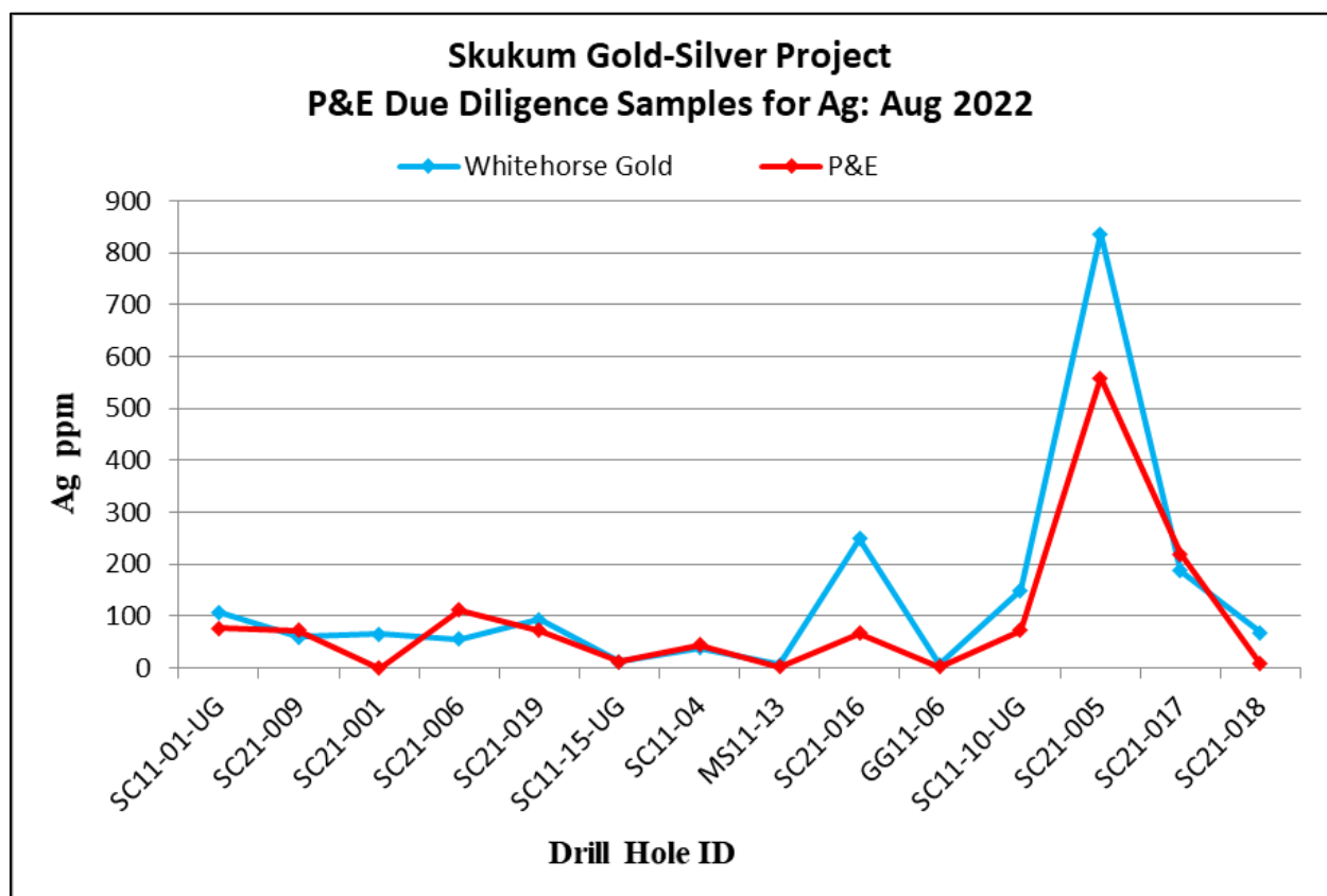
FIGURE 12.2 P&E SITE VISIT RESULTS: AG
