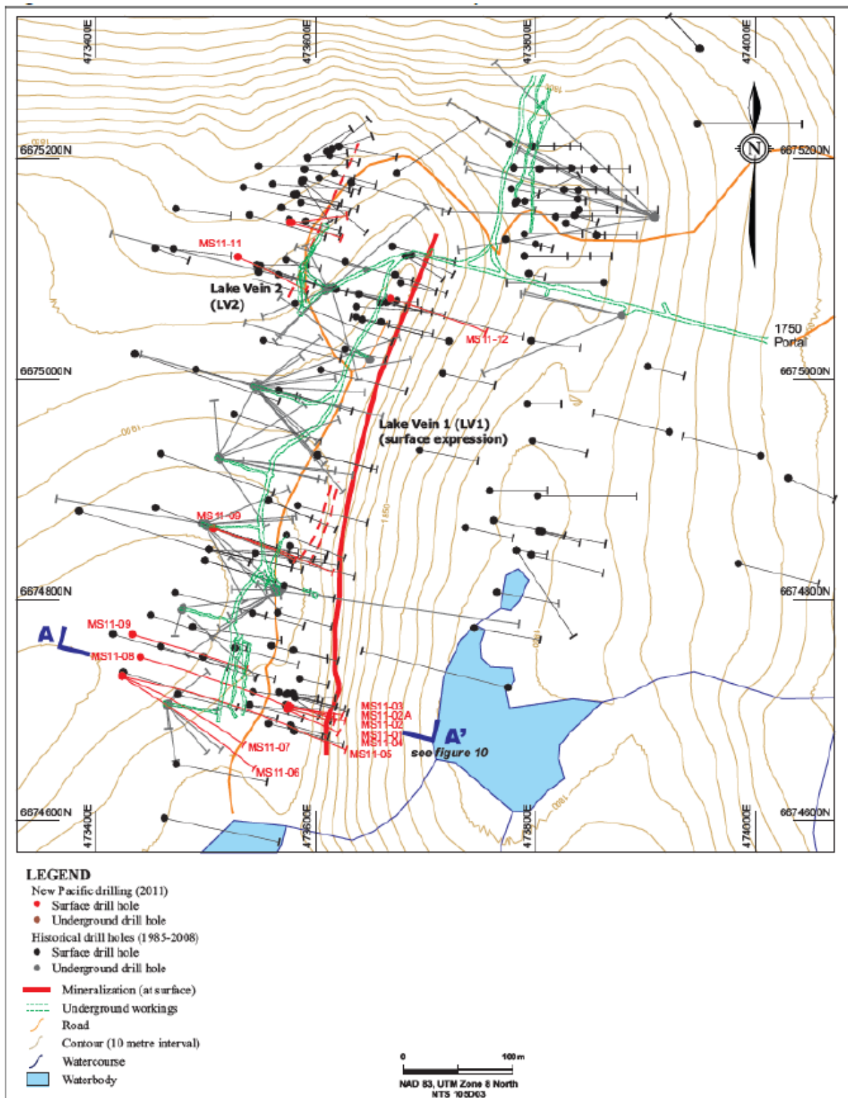
FIGURE 6.2 2011 DRILL HOLE PLAN, LAKE ZONE, MT. SKUKUM DEPOSIT
