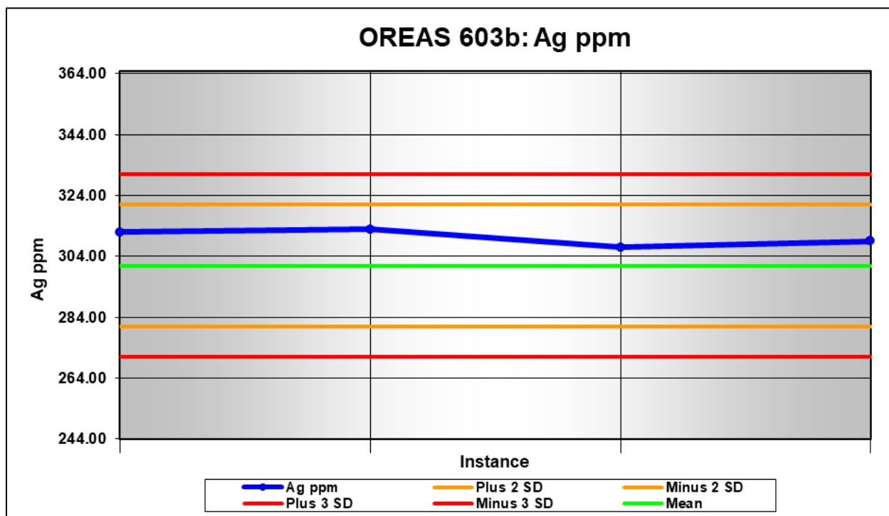
FIGURE 11.4 PERFORMANCE OF OREAS 603B CRM: AG
