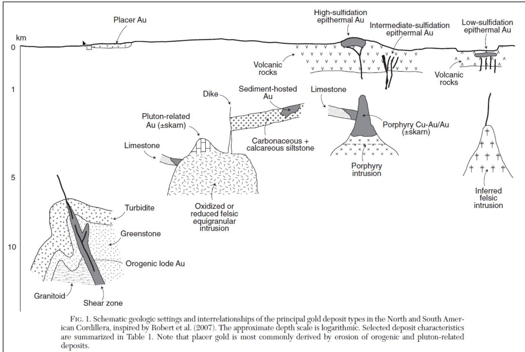
FIGURE 8.1 SCHEMATIC CROSS-SECTION OF THE MAIN GOLD MINERALIZING SYSTEMS AND CRUSTAL DEPTHS
