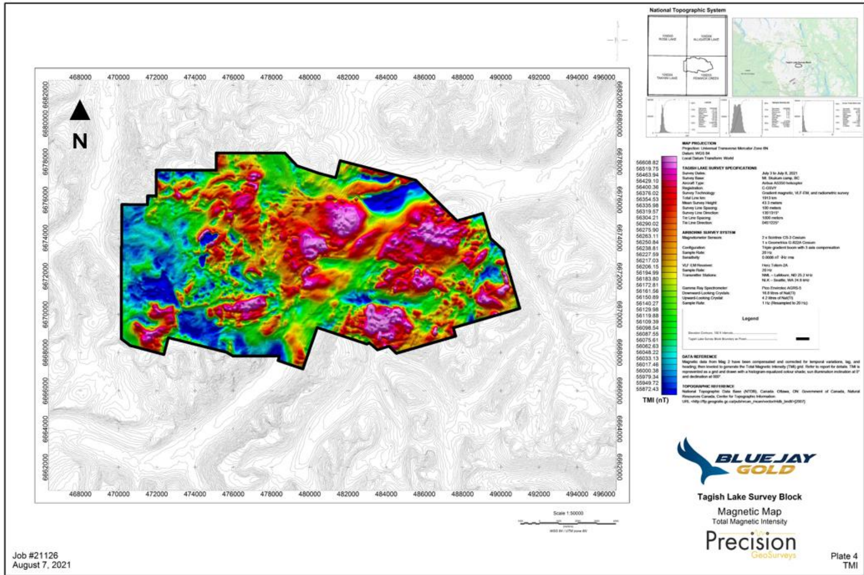
FIGURE 9.6 TOTAL AIRBORNE MAGNETIC INTENSITY MAP
